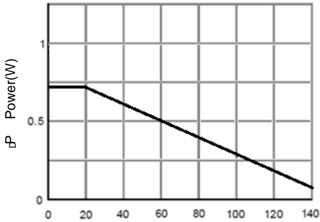
Figure 1 Power Dissipation
